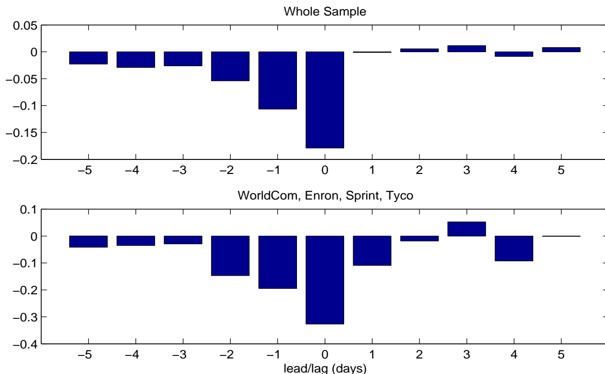
Figure 1: Cross Correlation of Stock Returns and CDS Changes.
